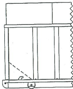
VIEW B - B HINGE SIDE VIEW
