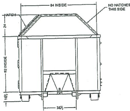
LIFT END VIEW
