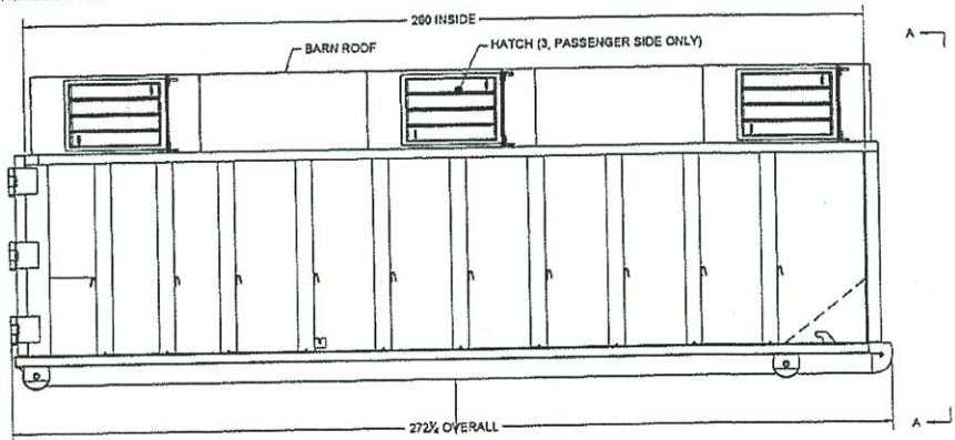
LATCH SIDE VIEW
